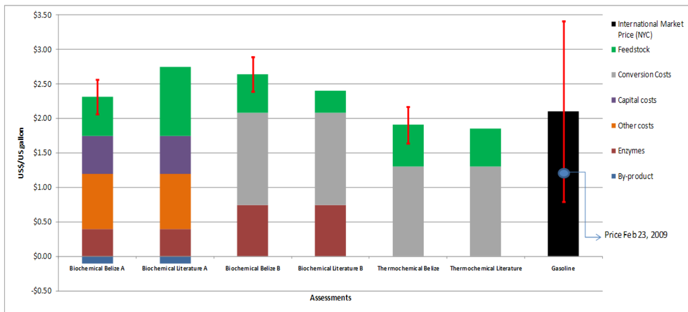
Figure 5 Cost breakdown comparison between Belize (error bars for uncertainty in feedstock costs) and literature reported CE production costs vs. Gasoline NYC international spot prices (average value from 2004-2009; uncertainty range represents the lowest and highest values in the market in the last 5 years)
