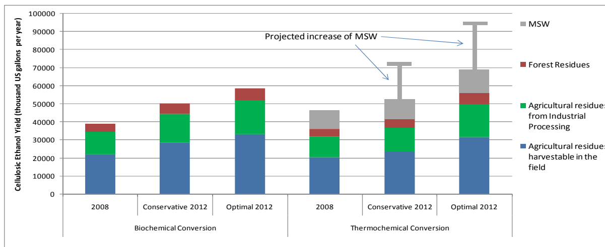
Figure 4 Cellulosic ethanol yields through Biochemical and Thermo-chemical conversions in 2008 and 2012 (conservative and optimal scenarios) by type of feedstock including projected increase of MSW
